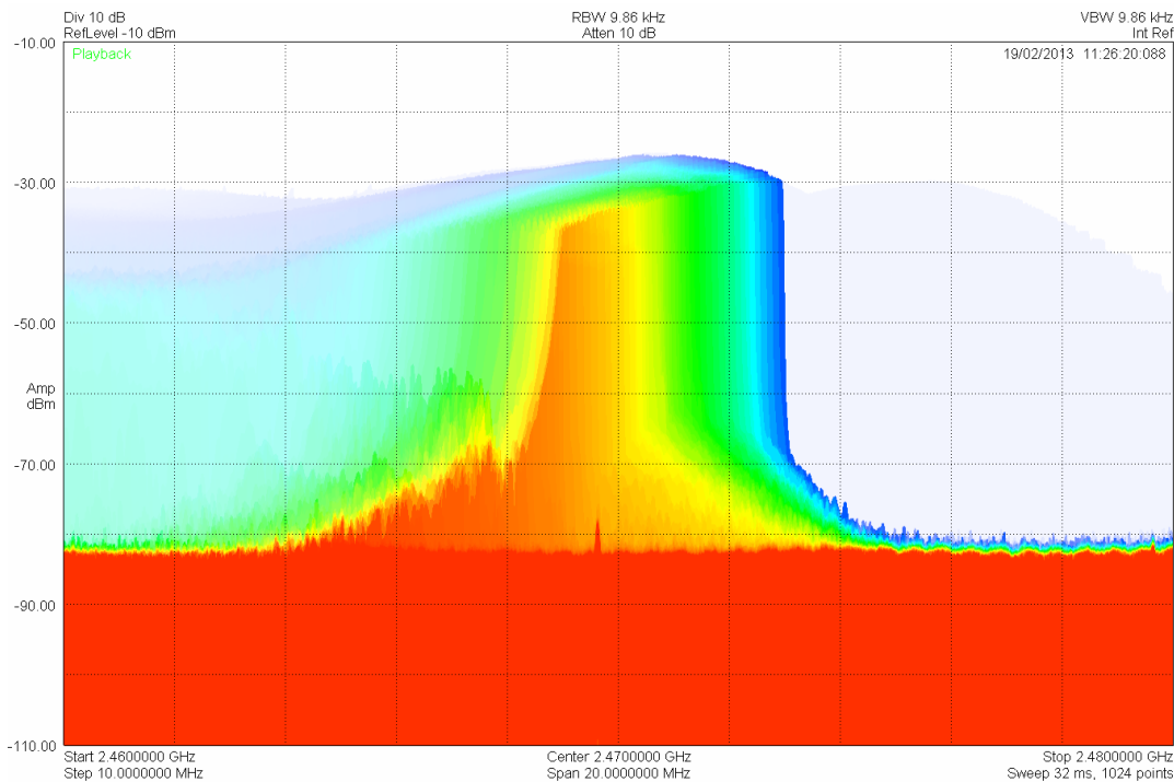
Figure 5: Sweep mode persistence showing the signal from a poorly shielded commercial microwave oven.
