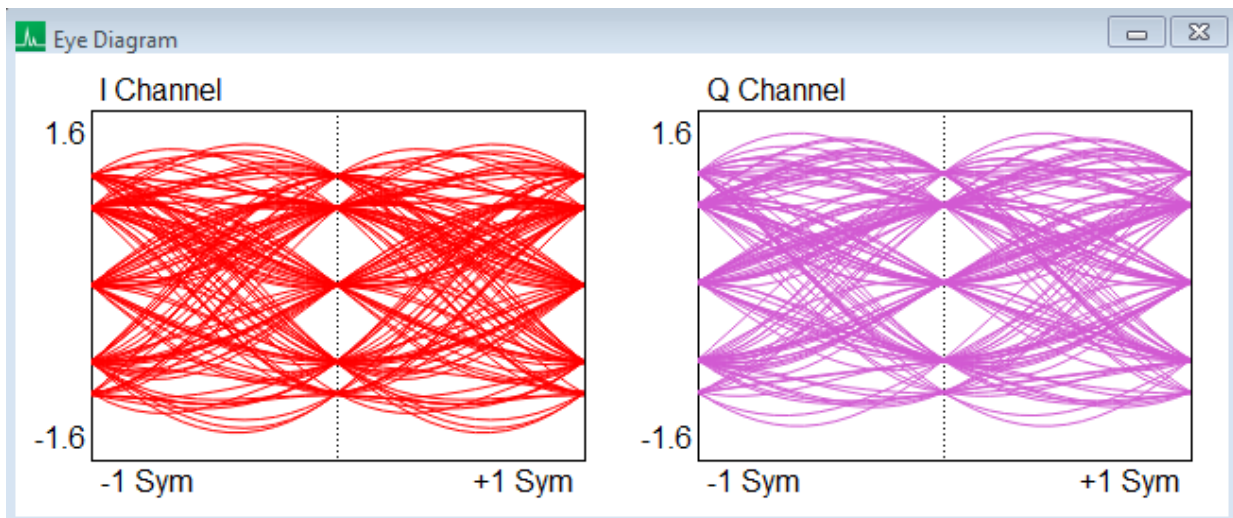
Figure 3: Eye diagram for a Pi/4DQPSK signal
