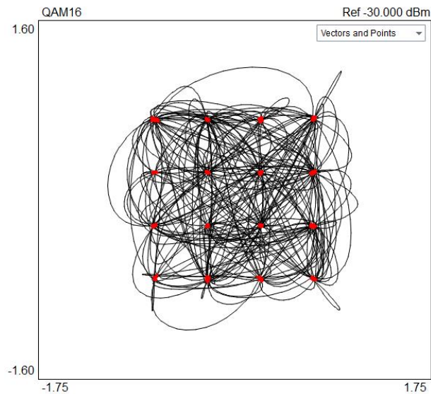
Constellation Diagram for a QAM 16 input signal
