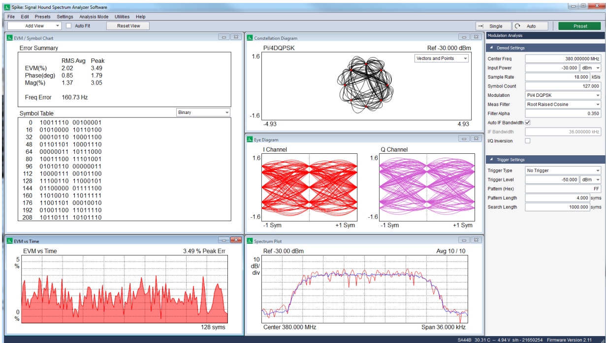
The SA44B demodulating a Pi/4QPSK signal
