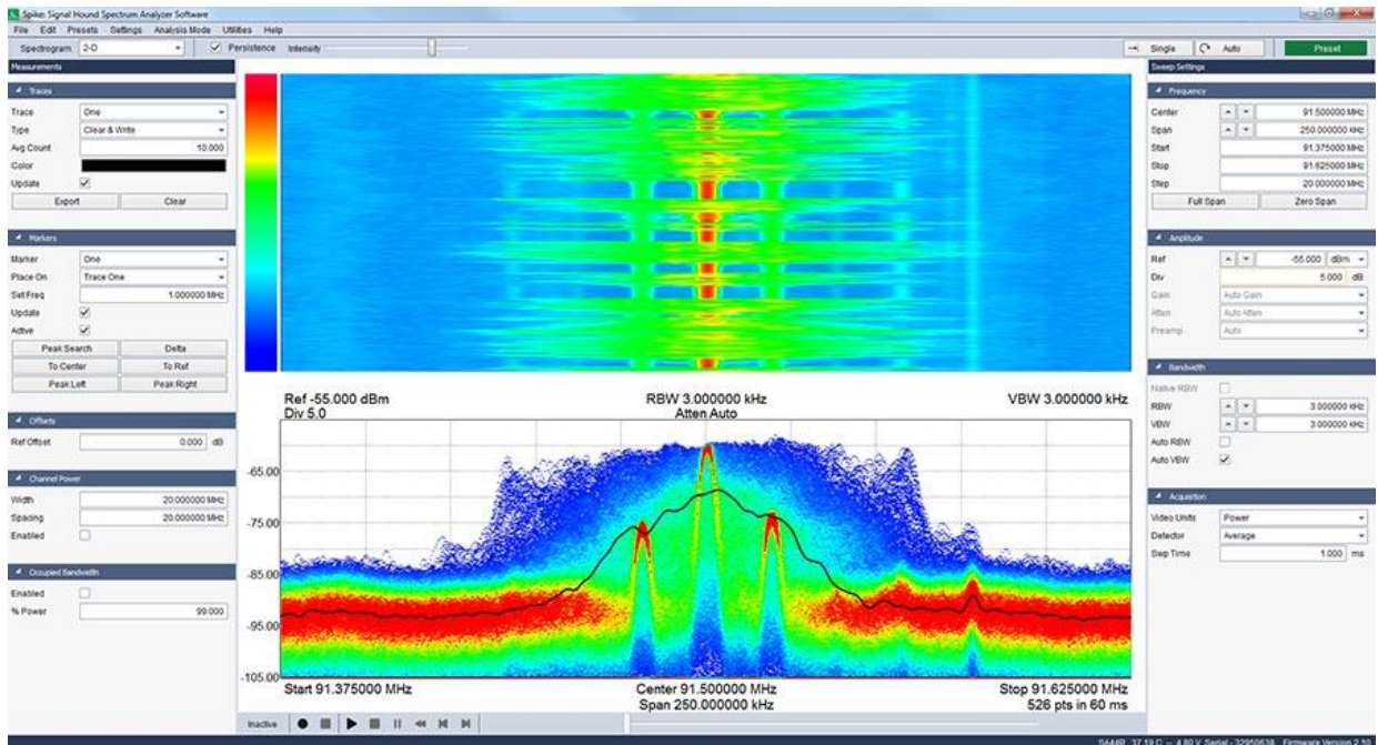
SA44B analyzing an FM radio station in real-time spectrum analysis mode. The persistence display is shown on the bottom half of the application and a 2-dimensional waterfall plot is shown on top.
